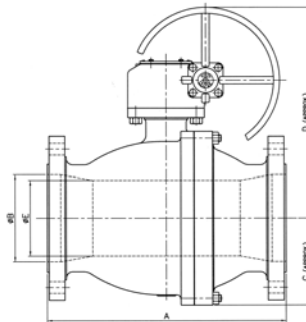
Reduced Bore Valve
