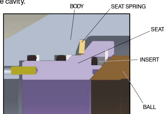
TMBV Seat design for Classes 150, 300 and 600 (Sealant Injection system for 8" valves and above)
