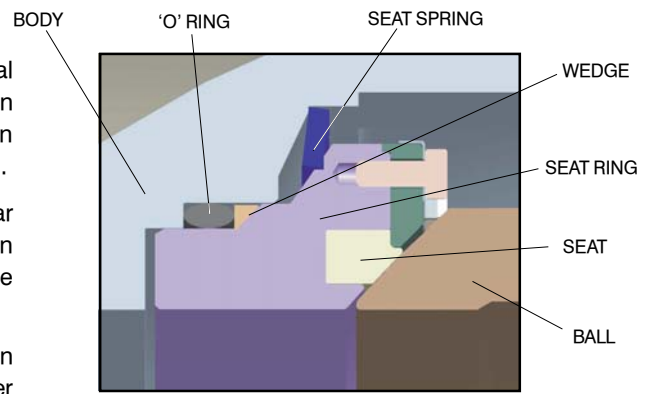
Seat design for Classes 150 and 300
