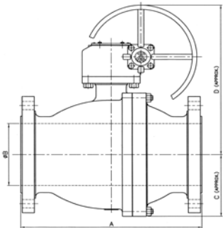
Full Bore Valve
