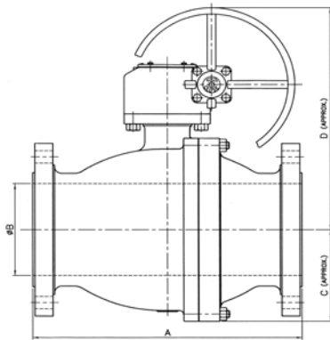
Full Bore Valve
